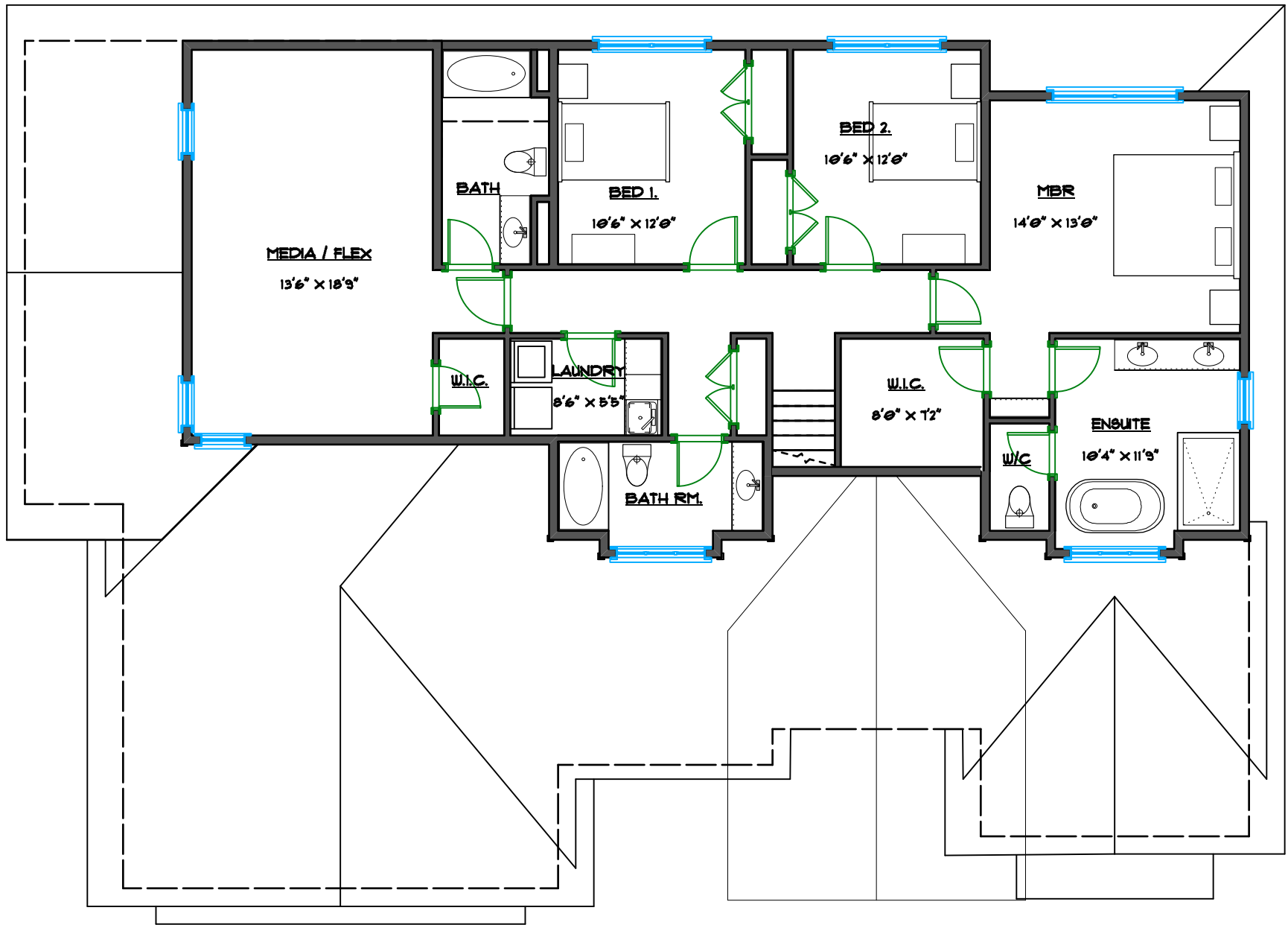
1 UPPER FLOOR PLAN SCALE: 1/8" = 1'-0" 1471.34 SQ.FT. (136.69 SQ.M.)
