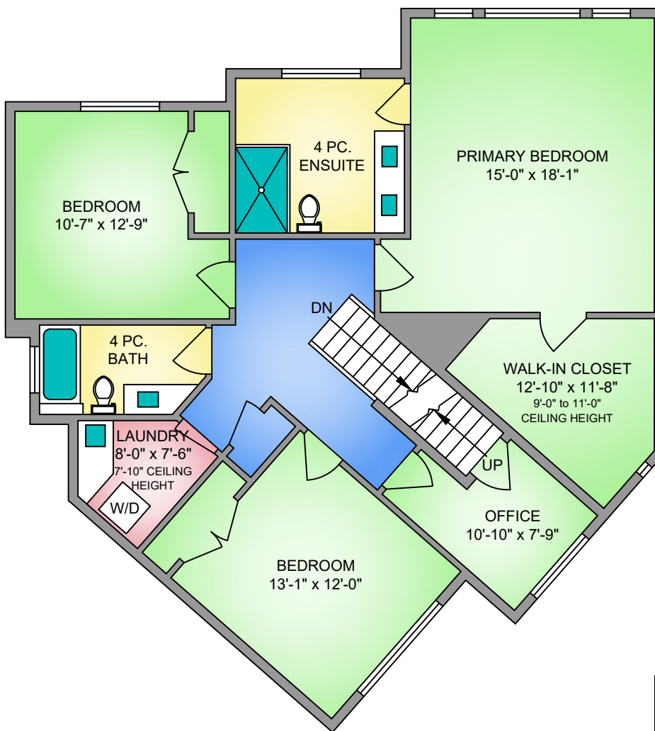
UPPER FLOOR 1307 SQ. FT. 7'-8" to 11'-0" CEILING HEIGHT
